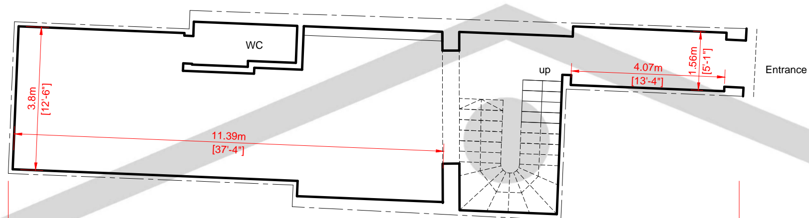
Ground floor level
