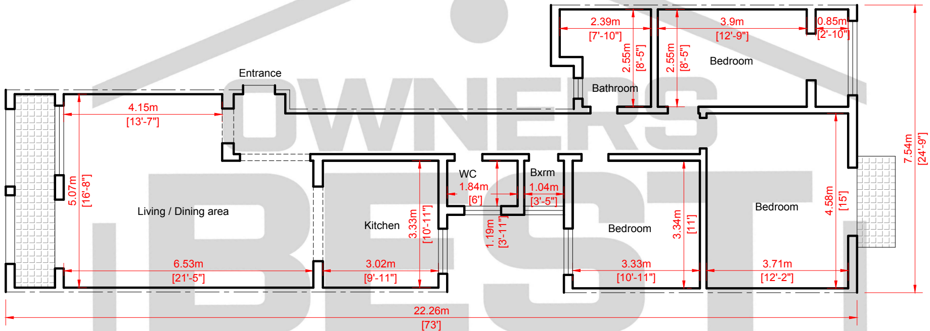
First floor level
